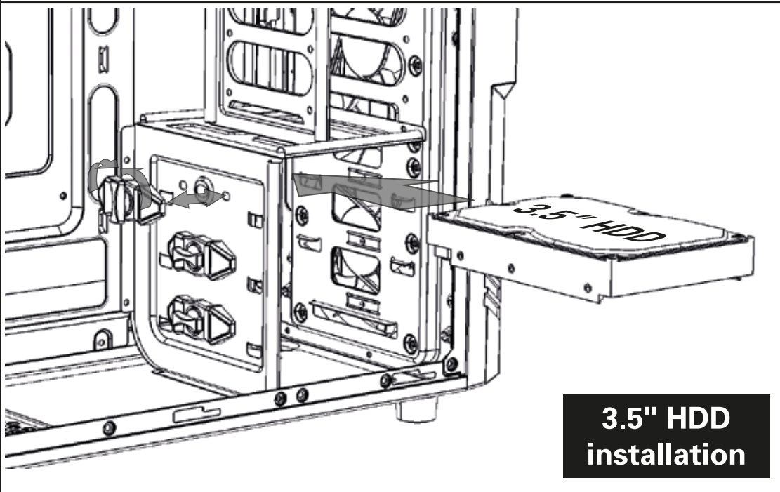
3.5" device installation
